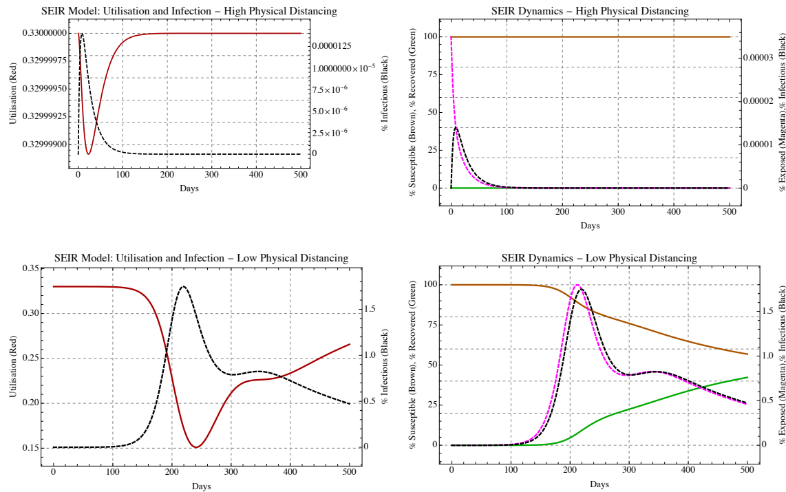
Figure 5: SEIR- u model: strong vs. weak physical distancing
