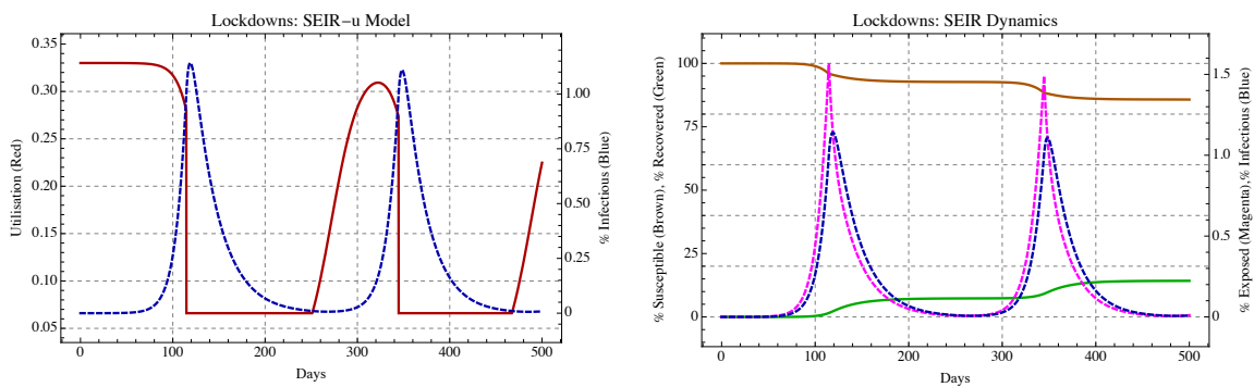
Figure 7: SEIR- u model: lockdowns
