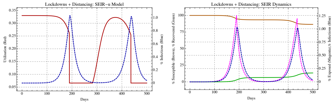
Figure 10: Lockdowns/physical distancing interactions.
