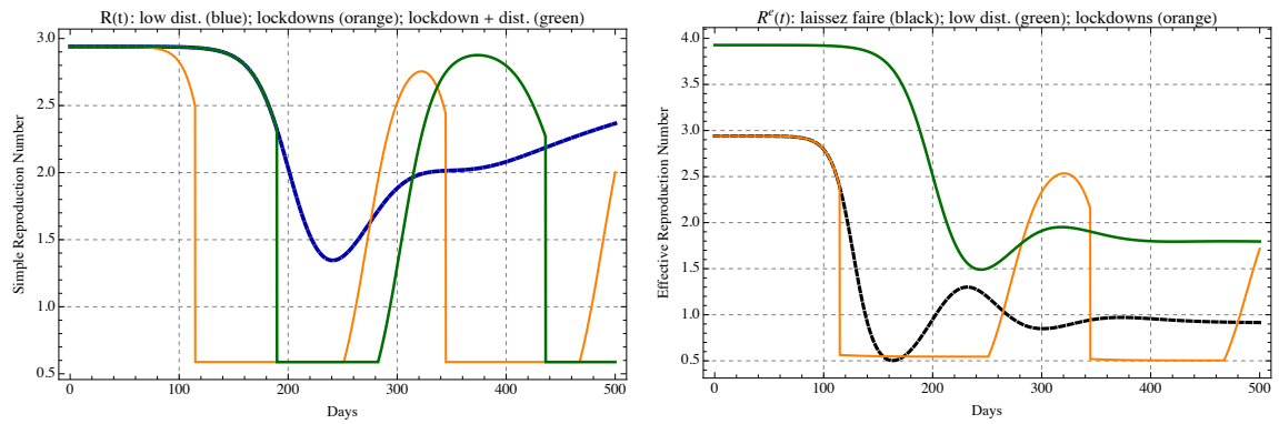
Figure 16: SEIR-u model: reproduction rates.
